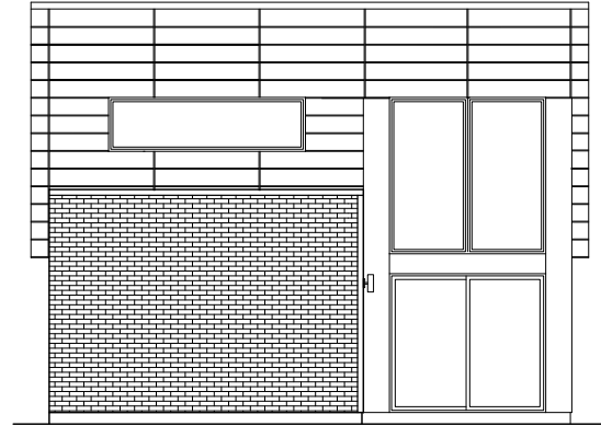
ELEVATION ARRIERE Echelle 1/4" = 1'-0"
